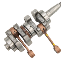
T8-05020100 Fits:PARSUN T8/9.8 3B2-00030-1 Fits:Tohatsu M6B/8B/9.8B
